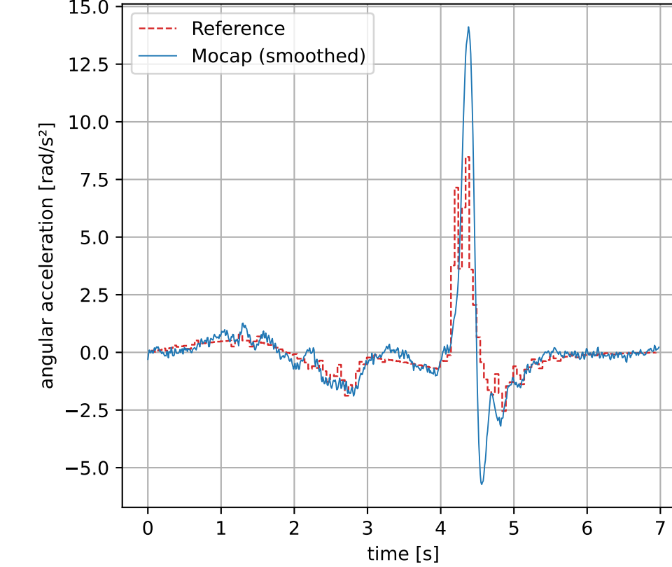
Angular Acceleration
